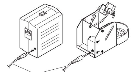
Connecting cable
